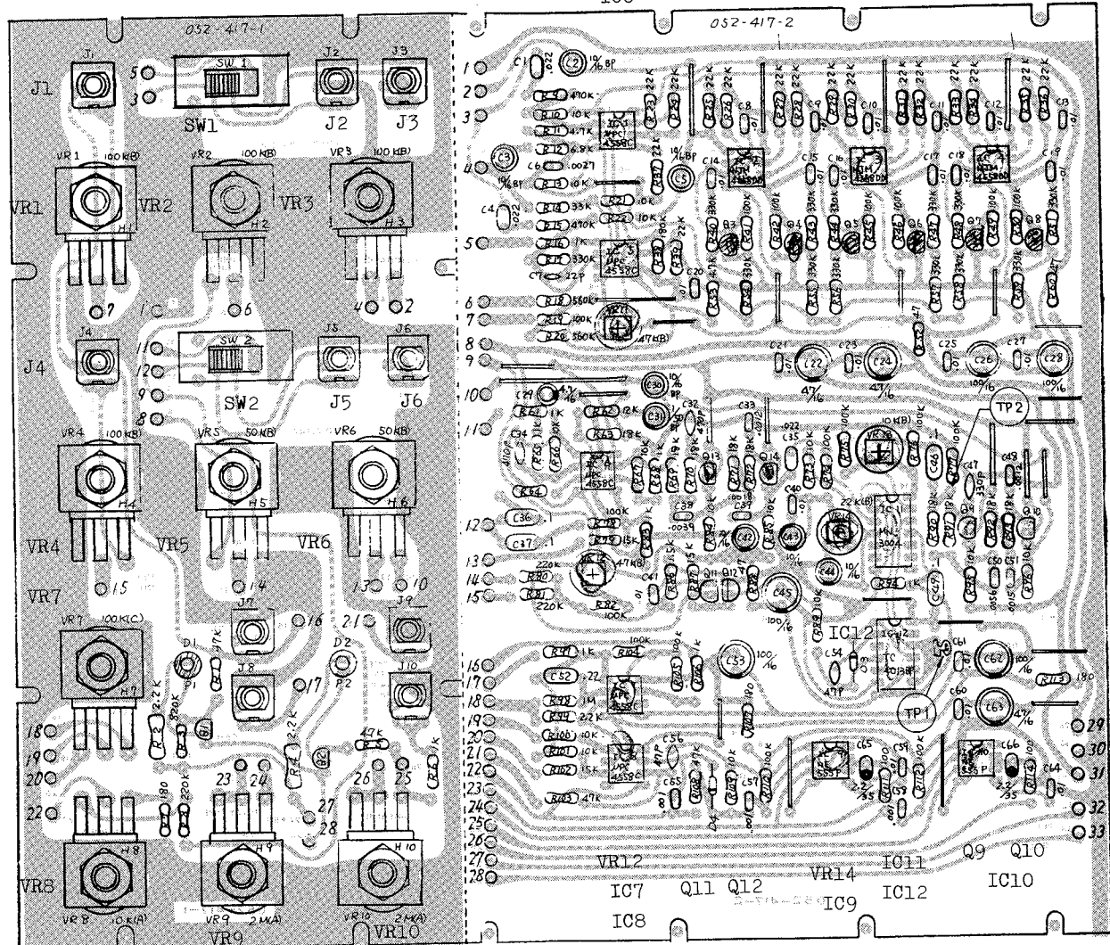
OP9109-040 (Part number 7910904000) (pcb 052-417-2)
